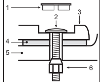
MOUNTING HARDWARE
