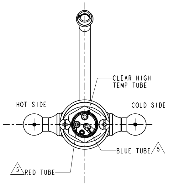
BOTTOM VIEW SCALE .375
