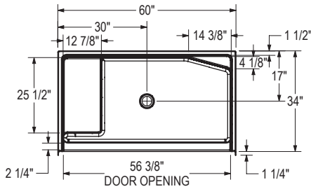
STANDARD MODEL (Left Seat Shown)
