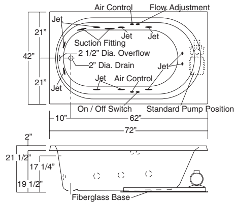
10-jet Bodywrap System ACOV-4272 / BWS (illustrated)
