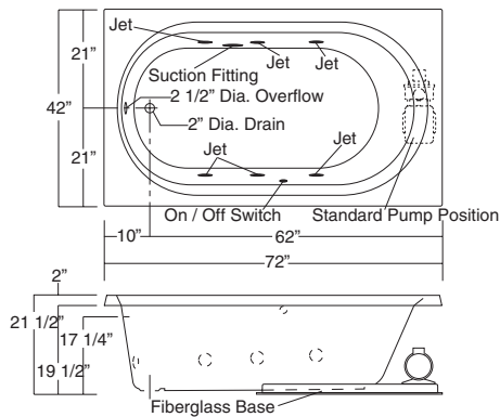
6-jet Homestead Collection ACOV-4272 / HMS (illustrated)
