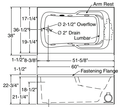
6-jet Homestead System SBA-3260L / HMS (illustrated)
