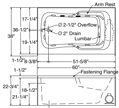
10-jet Bodywrap System SBA-3260L / BWS (illustrated)
