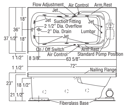
10-jet Bodywrap System SBF-3672L / BWS (illustrated)
