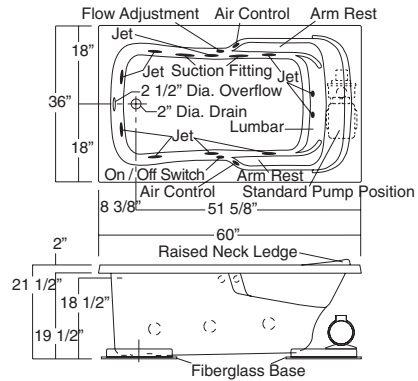
10-jet Bodywrap System SB-3660 / BWS (illustrated)
