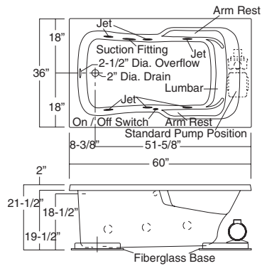
6-jet Homestead Collection SB-3660 / HMS (illustrated)
