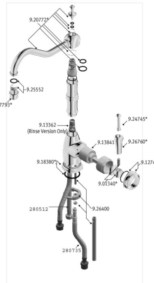
11" Spout U.4747-2
