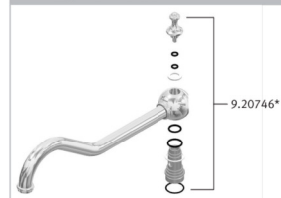
Bar Spout
