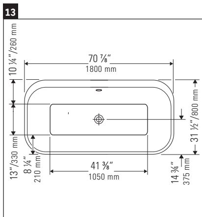
Measurements for Happy D.2 Plus.
