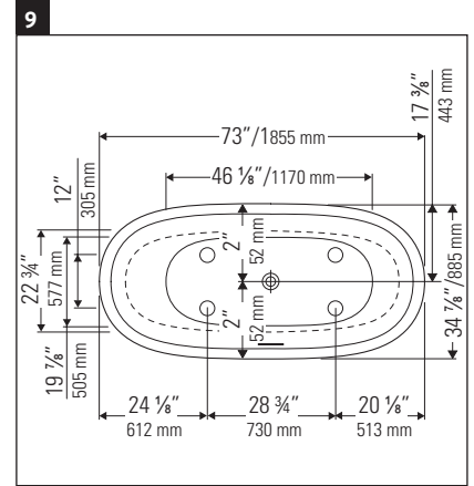
Measurements for Cape Cod.
