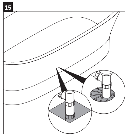
> Remove installation aids. > Connect bathtub to drain system.
