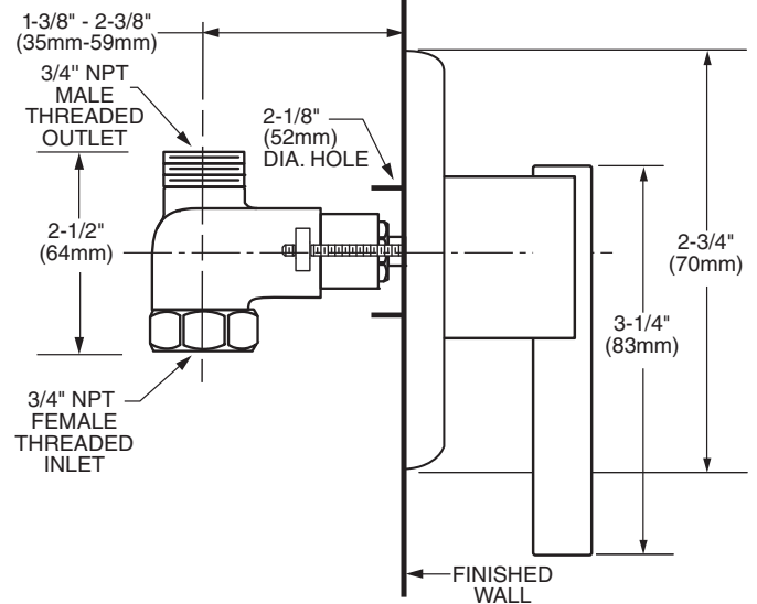
Model R711 3/4" NPT
