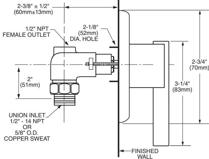
Model R701 1/2" NPT
